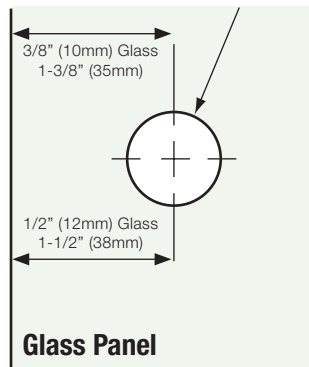
Overlapping Panel
