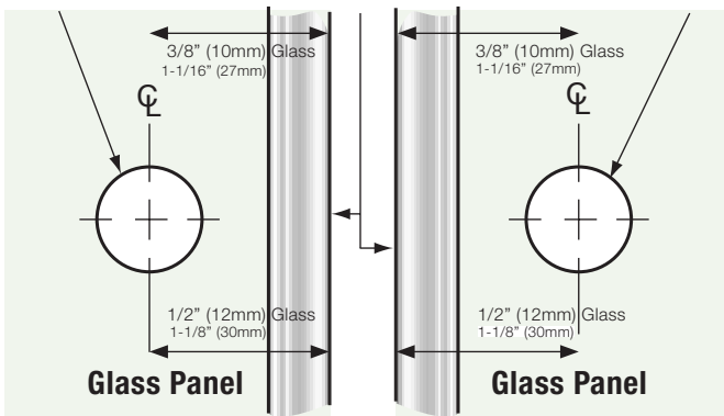
22.5° Mitered Panel
